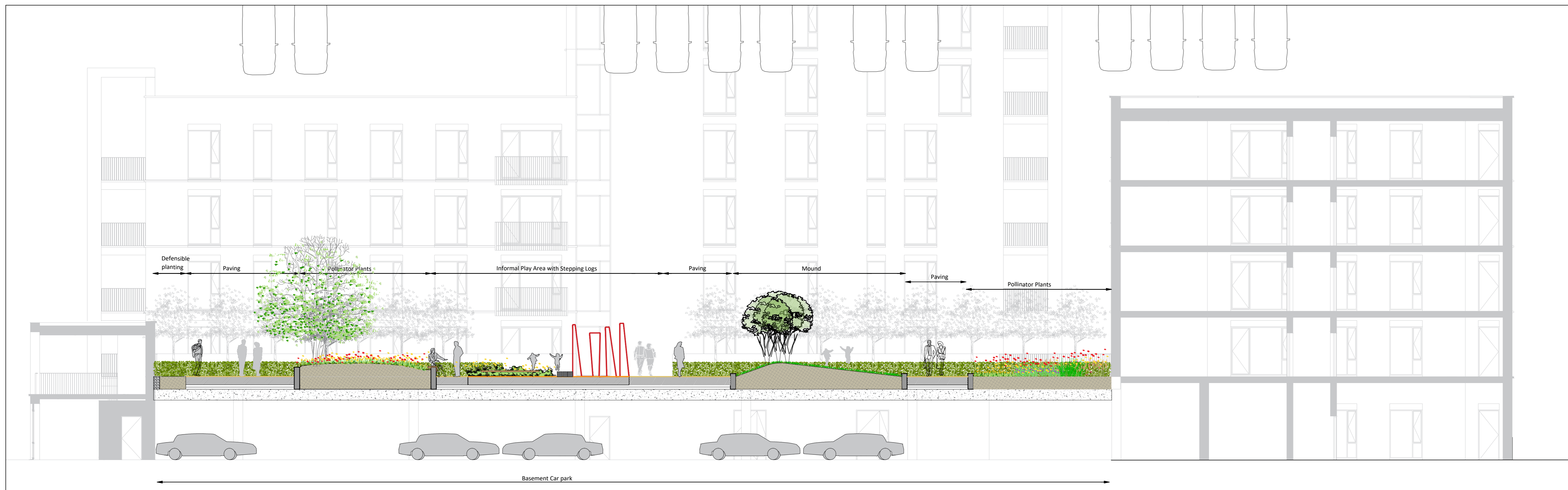
SECTION A-A - THROUGH PODIUM BLOCK A Scale 1: 100
